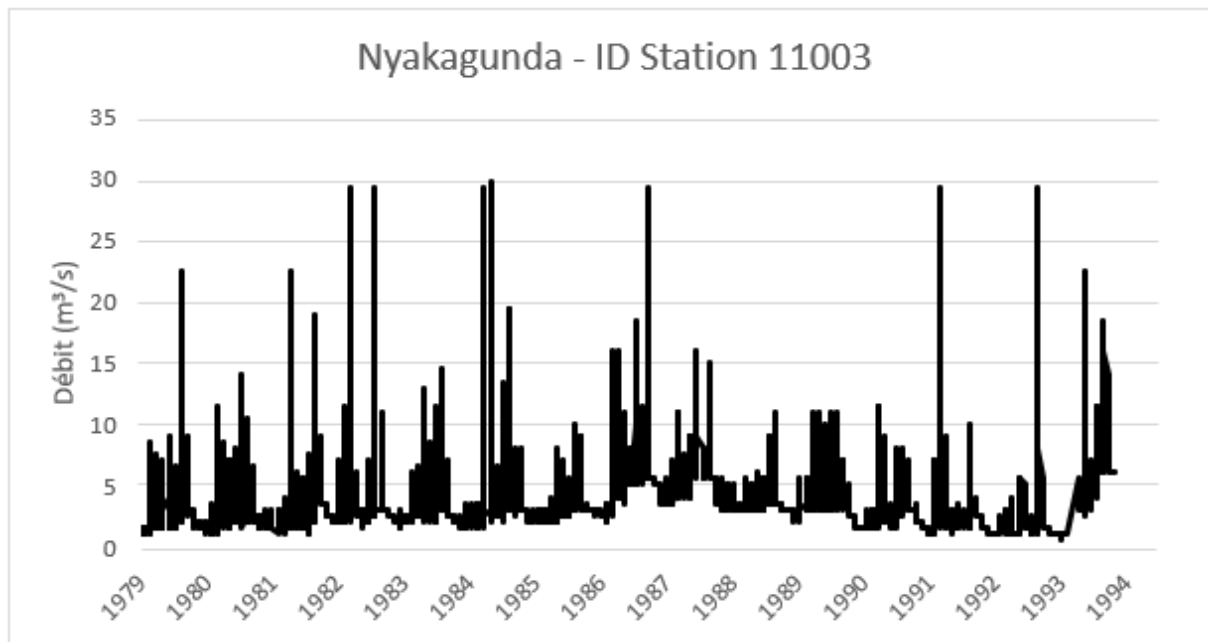
Appendix 2 - 011 - Hydrograph of the Nyakagunda River (11003), according to IGEBU data
