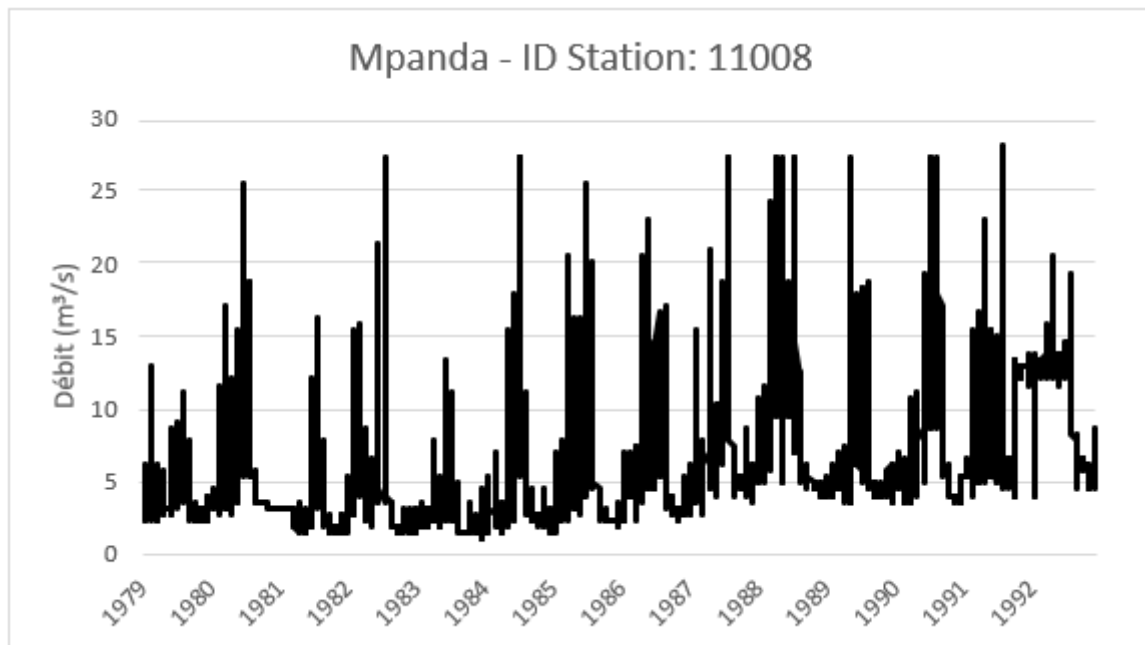
Annex 2 - 010 - Hydrograph of the river Mpanda (11008), according to IGEBU data
