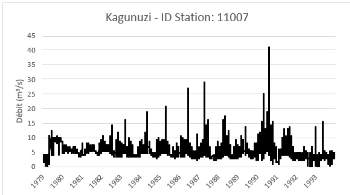
Appendix 2 - 009 - Hydrograph of the Kagunuzi River (11007), according to IGEBU data
