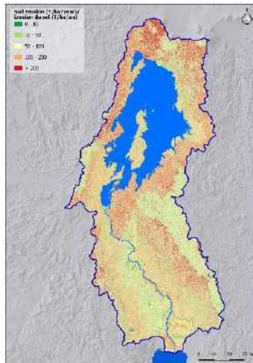
Figure 31: Map of RUSLE in t/ha/year.
